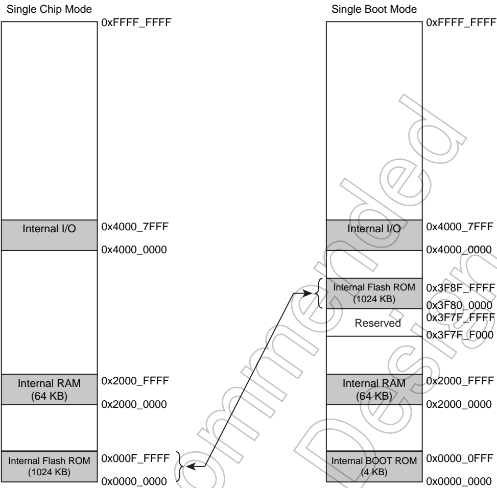
Figure 24-3 Memory Maps for TMPM364F10FG
