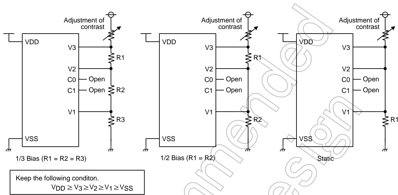
Figure 13-4 Connection Examples When Using an External Resistor Divider (LCDCR<BRES> = "0")
