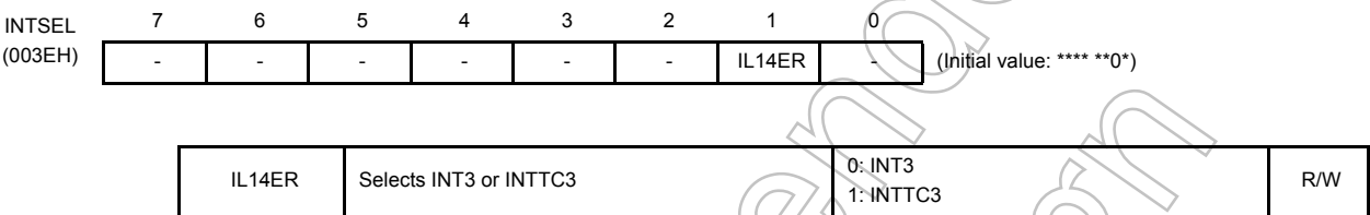
Interrupt source selector
