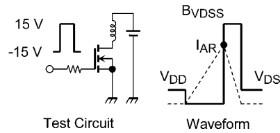
Fig. 8.16 Test Circuit/Waveform
