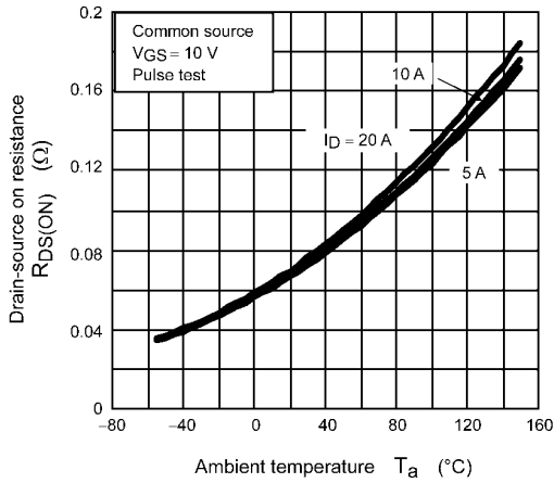
Fig. 8.7 R_{DS(ON)} - T_a
