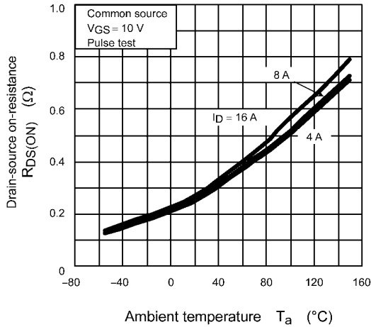
Fig. 8.7 R_{DS(ON)} - T_a
