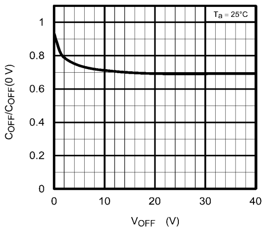
図 12.1.11 C_{OFF}/C_{OFF}(0V) - V_{OFF}
