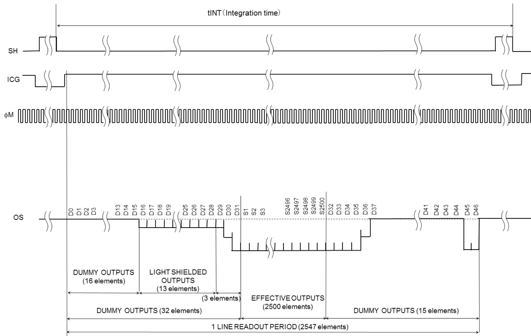
Timing Chart 1
