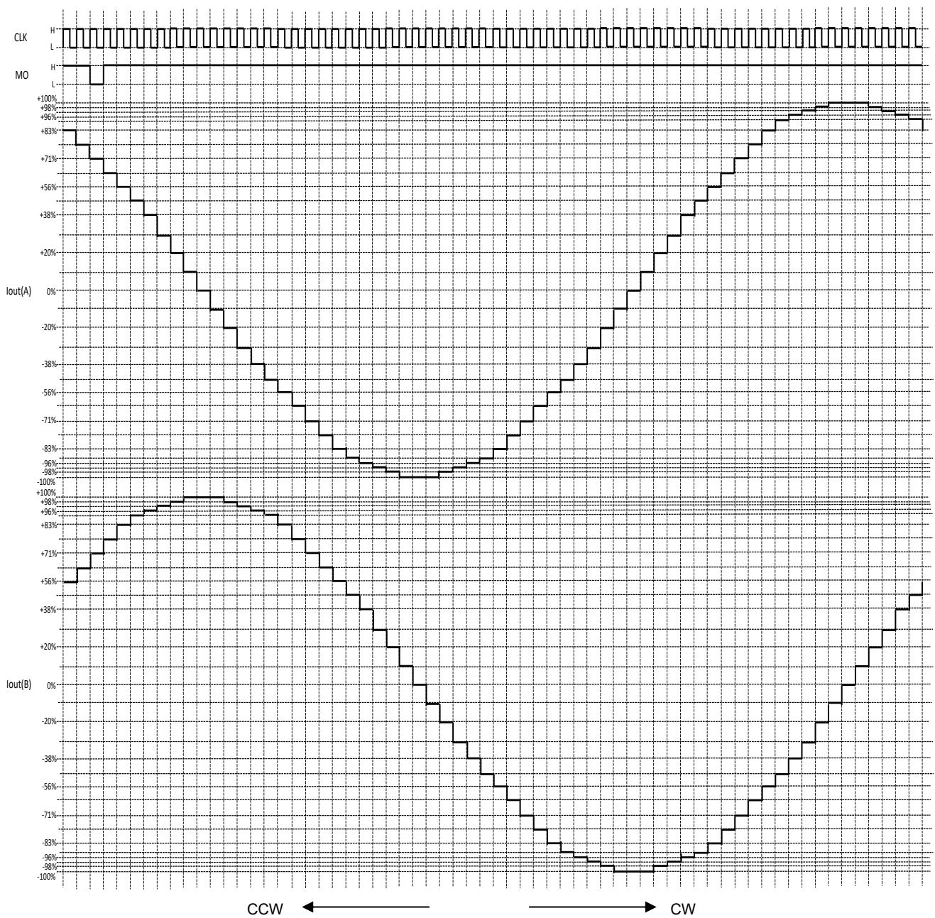
Figure 6.6 1/16 step resolution
