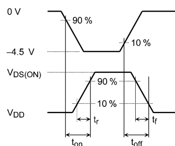
Fig. 6.3.2 Input Waveform/Output Waveform
