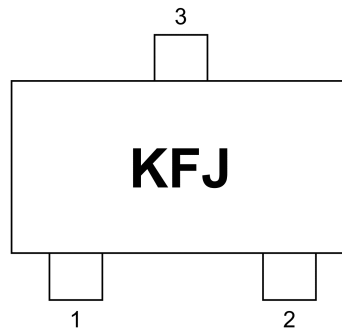
Fig. 7.1 Marking
