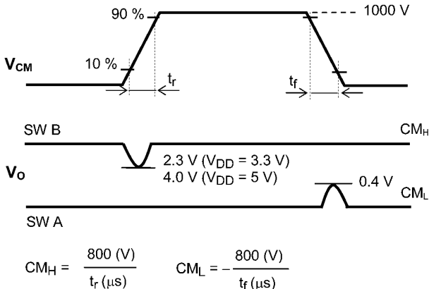
Fig. 12.1.7 Common-Mode Transient Immunity Test Circuit and Waveform
