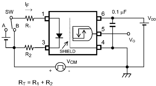
Fig. 12.1.7 Common-Mode Transient Immunity Test Circuit and Waveform
