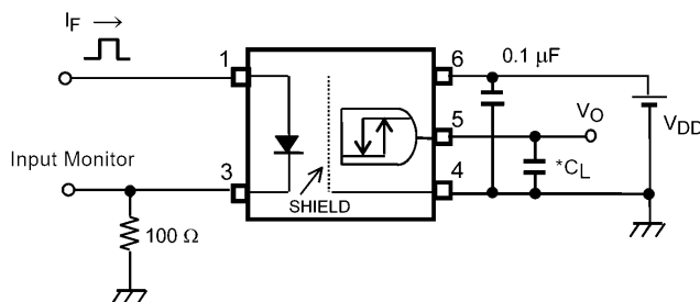
Fig. 12.1.6 Switching Time Test Circuit and Waveform
