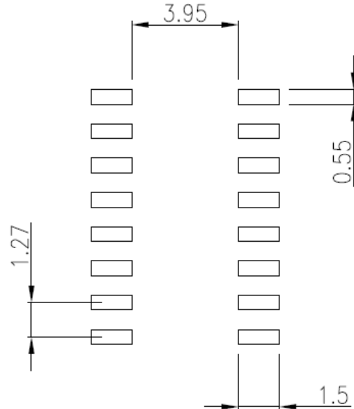
TBD62502AFG, TBD62503AFG
