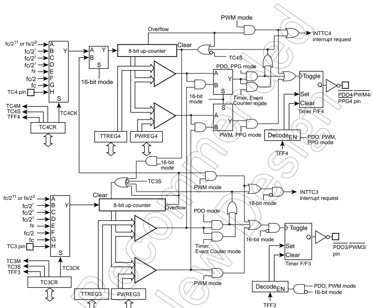
Figure 9-1 8-Bit TimerCounter 3, 4
