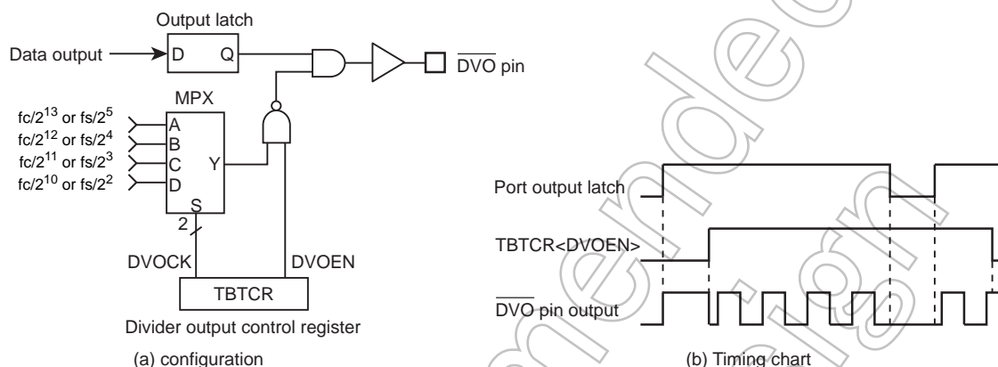
Figure 5-3 Divider Output
