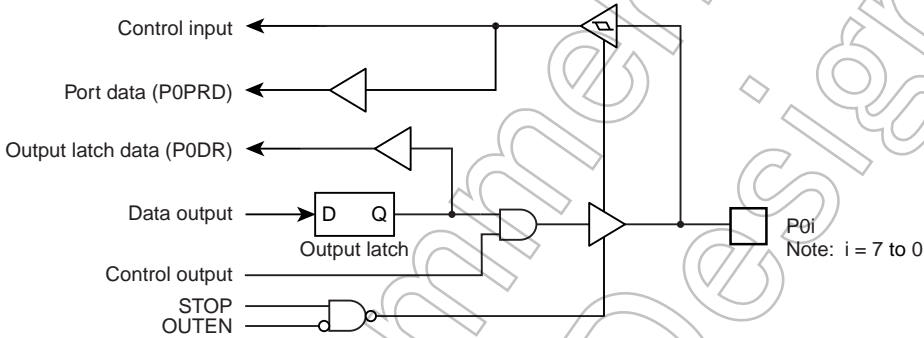
Figure 7-2 Port 0
