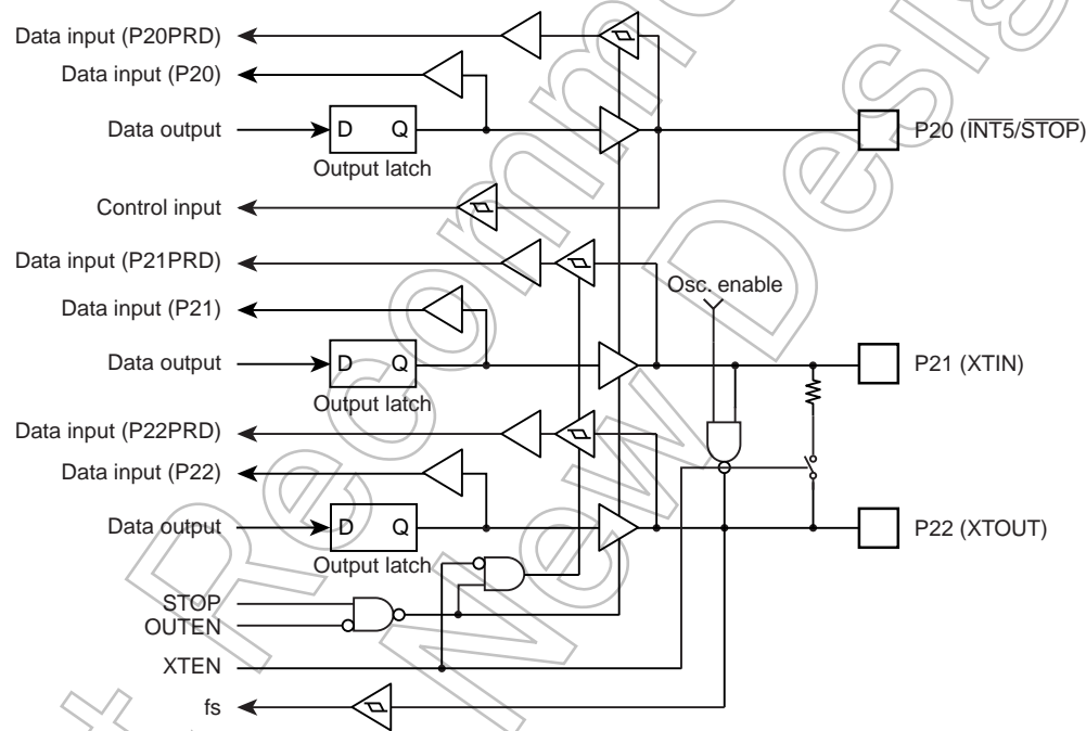
Figure 7-4 Port 2
