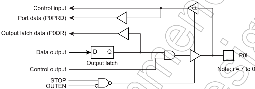
Figure 7-2 Port P0
