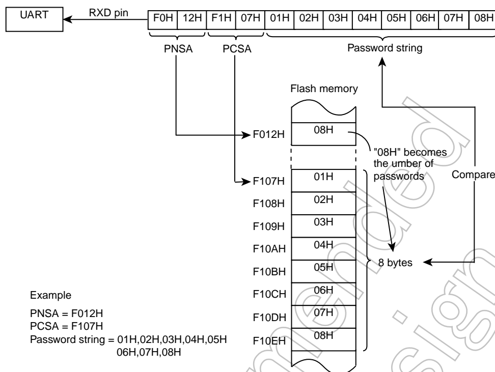
Figure 15-5 Password Comparison
