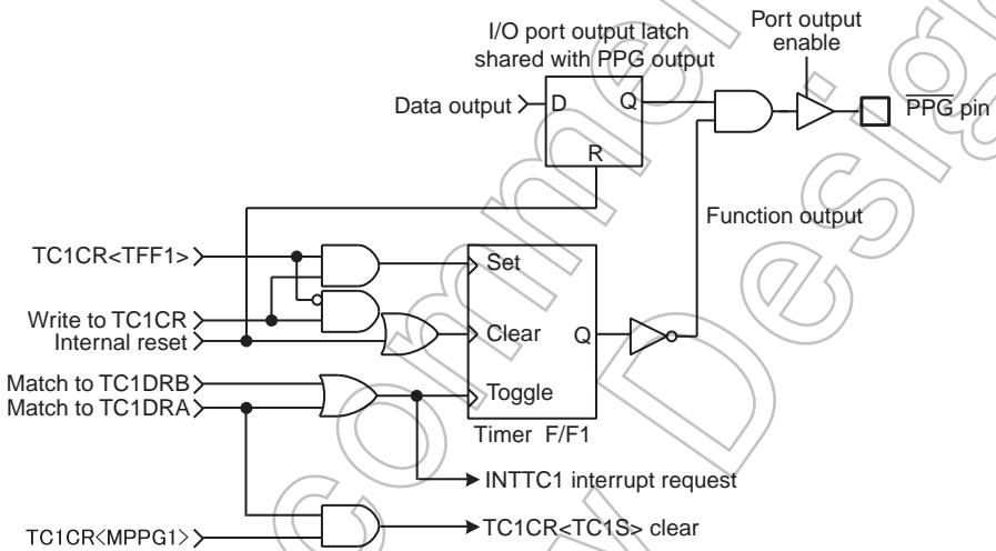
Figure 8-7 PPG Output
