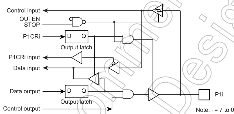
Figure 7-3 Port P1
