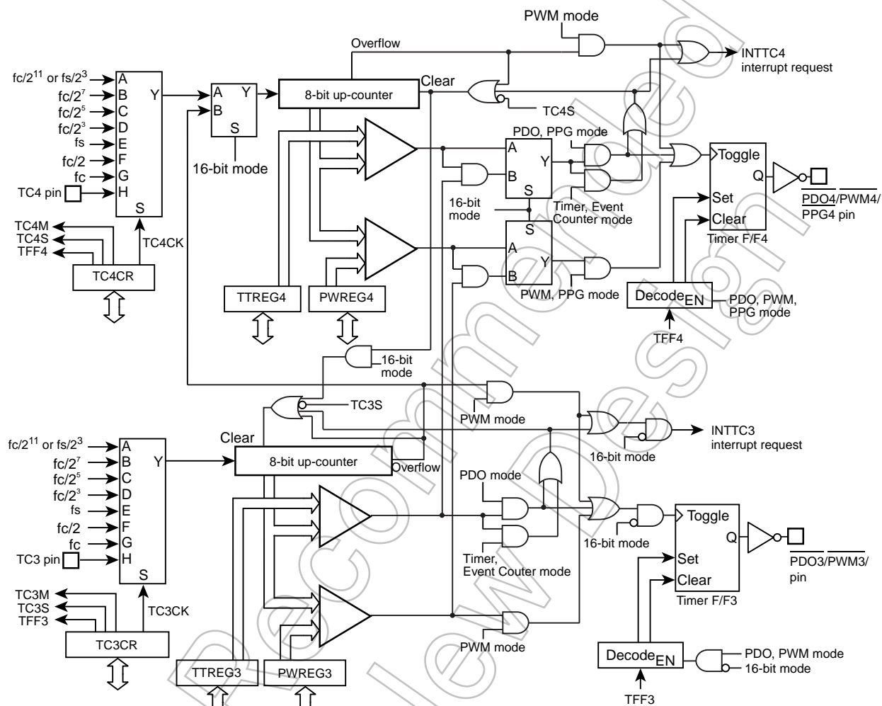
Figure 9-1 8-Bit TimerCounter 3, 4
