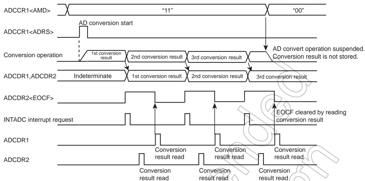
Figure 12-3 Repeat Mode
