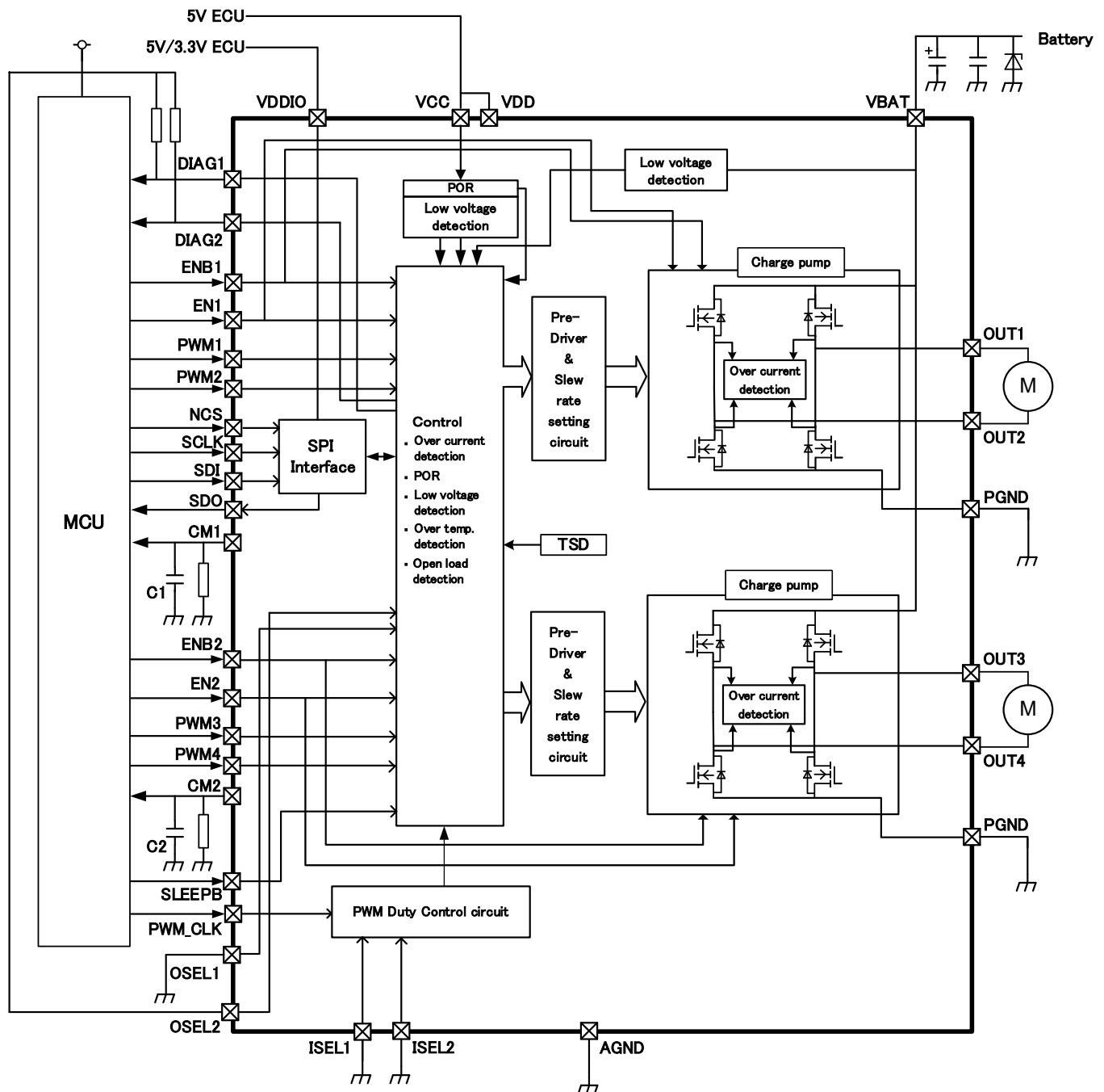
Figure 4.1. Block diagram
