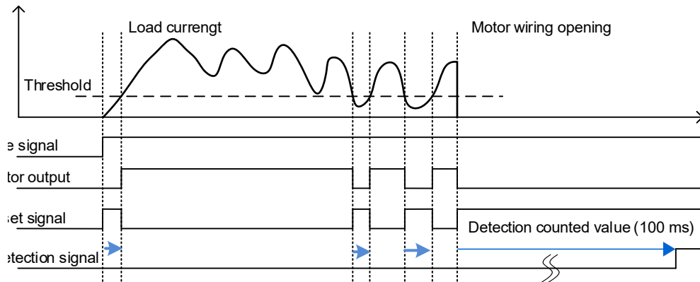
Figure 7.23 Open-load detection during operation: operation waveform
