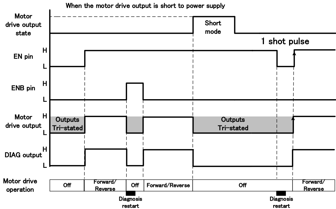
Figure 7.45 Recovery from OFF state for short-circuit to power supply or ground, and short-circuited load: timing chart
