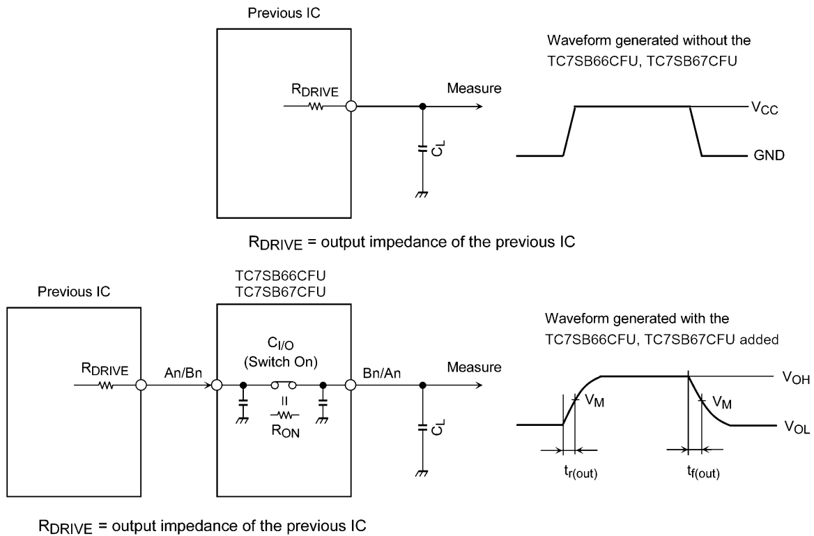
Fig. 12.1 Calculation Circuit
