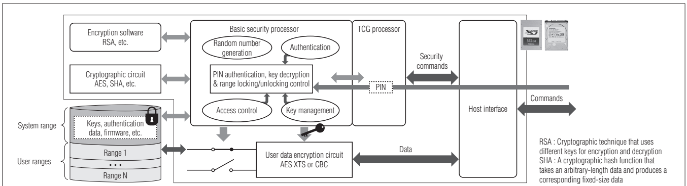
Fig. 2 Configuration and personal identification number (PIN) authentication of HDD and SSD — User authentication, key allocation and range locking/unlocking are performed using PINs.
