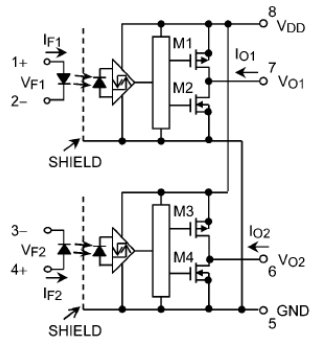
Internal circuit configuration (TLP2210)
