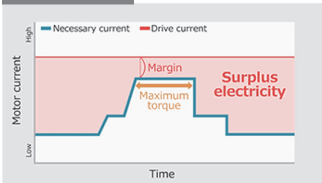
Open-loop control
