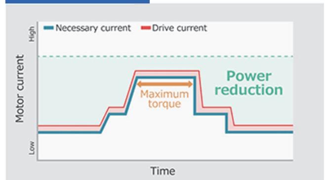
Active Gain Control (AGC)
