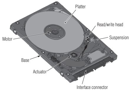
Figure 1 Internal structure of MQ02ABF100 — The MQ02ABF100 provides a capacity of 1 Tbyte in a 7 mm-thick casing by using a newly developed thin platform, a thin spindle motor, and a base optimally shaped through shock analysis.
