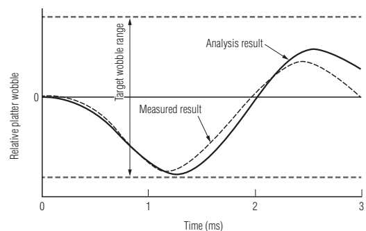
Figure 5 Result of analysis and measured data of disk amplitude when shock applied —
