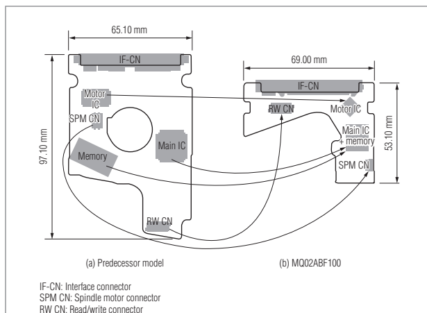
Figure 6 Reduction of printed circuit board —
