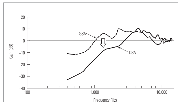
Figure 8 Comparison of servo compression characteristics of single-stage actuator (SSA) and DSA —
