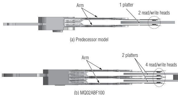
Figure 2 Comparison of structure and disk of conventional model and MQ02ABF100 —
