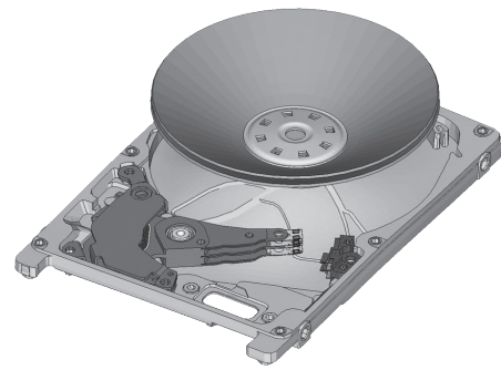
Figure 3 Example of result of shock analysis using finite element model — An FEM-based shock analysis was performed to optimize the base shape and thereby minimize the wobbling of disk platters due to shock application.
