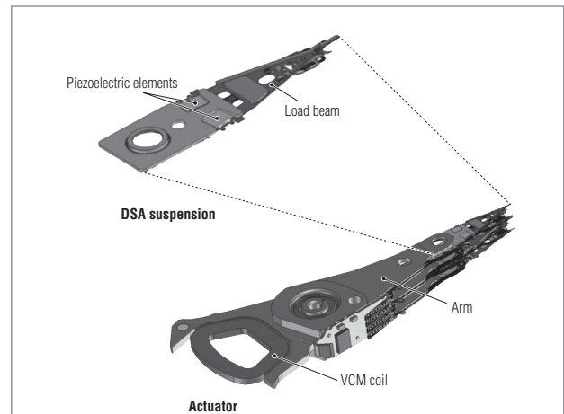
Figure 7 Newly developed actuator with DSA suspension —
