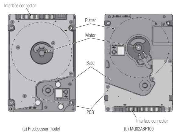
Figure 4 Comparison of base shape of predecessor model and base shape optimized for MQ02ABF100 —
