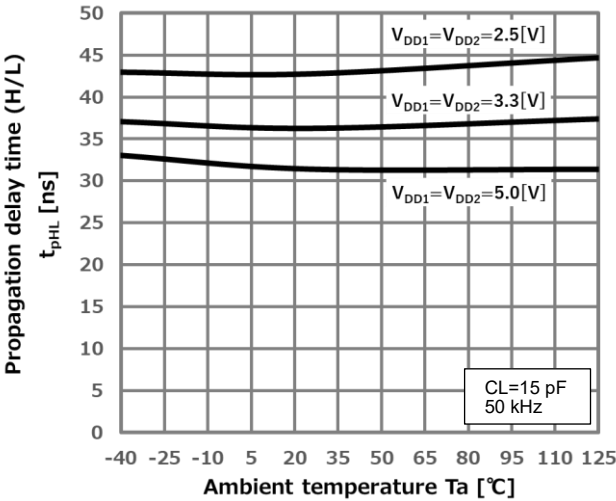
Fig.13.10. Propagation Delay Time t_{pHL}-T_a
