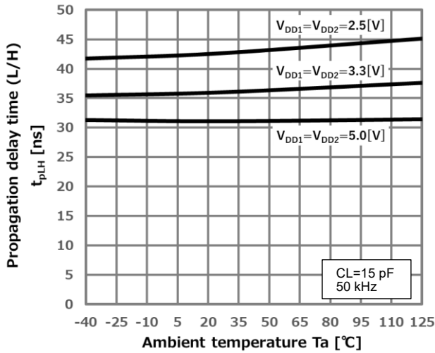
Fig.13.9. Propagation Delay Time t_{pLH}-T_a
