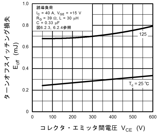
図 8.14 E_{\text{off}} - V_{\text{CE}}
