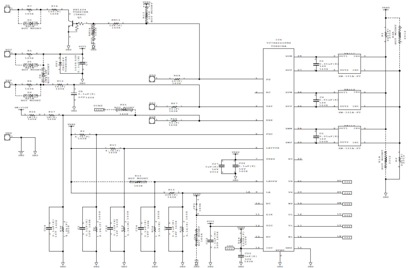
Figure 3.3 peripheral circuit of TC78B043FNG
