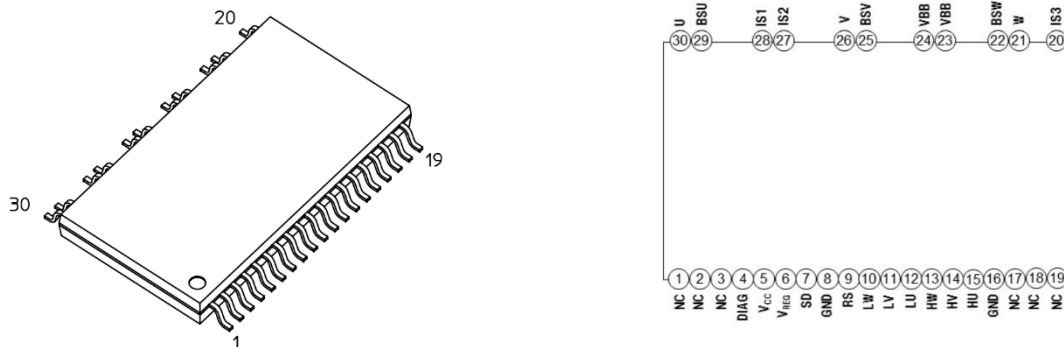
Figure 2.1 Appearance and Pin Assignment of TPD4204F
