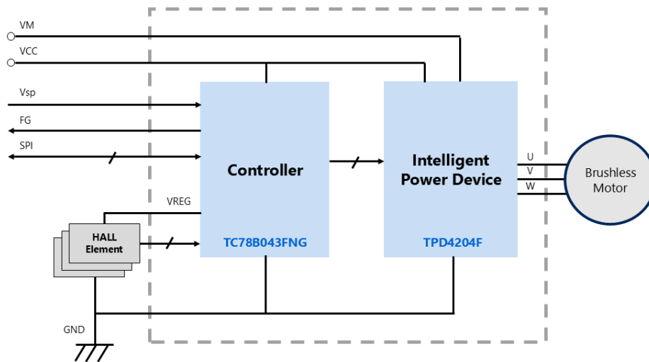
Figure 2.1 Block Diagram
