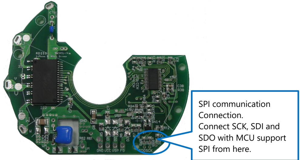
Figure 4.4 SPI Communication Connection
