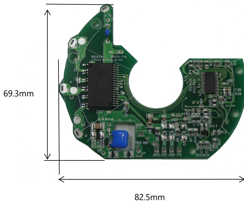
Figure 2.2 Board Appearance
