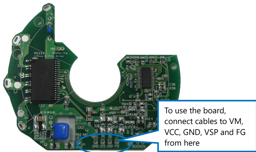
Figure 4.3 Layout of VM, VCC, GND, VSP, and FG connections
