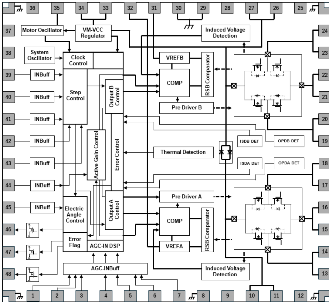
Figure 5.1 Block diagram
