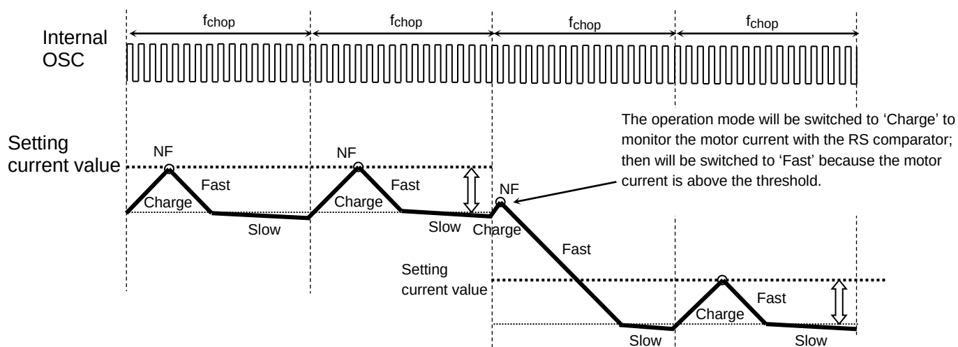
Figure 14.3.3 When the next current step is lower
