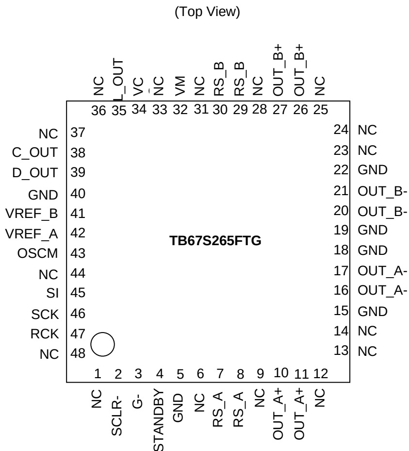
Figure3 Pin assignment
