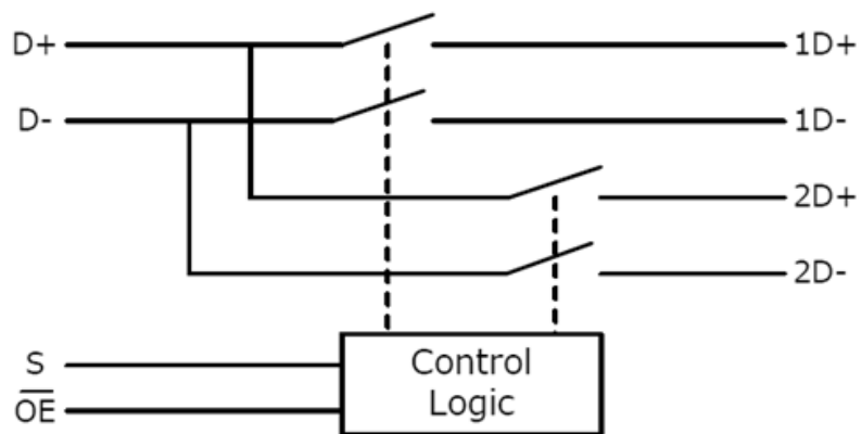
Fig. 6.1 Block Diagram
