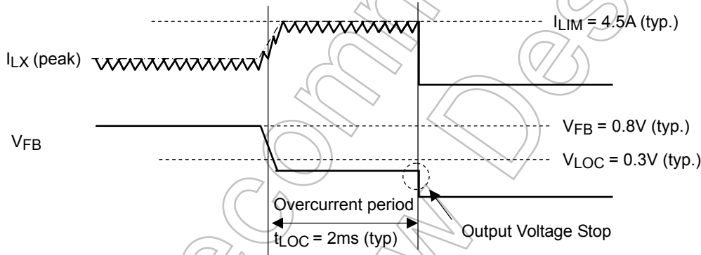
Figure 4 Overcurrent Operation
