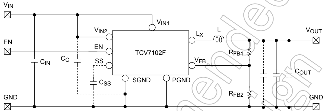
Figure 1 TCV7102F Application Circuit Example
