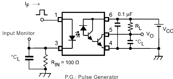
Fig. 12.1.1 Switching Time Test Circuit and Waveform
