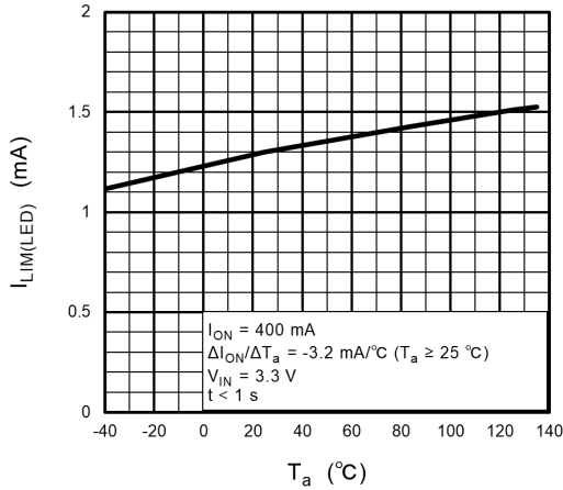
Fig. 12.7 I_{LIM(LED)} - T_a
