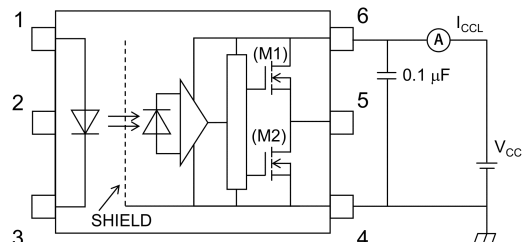
Fig. 13.1.6 I_{CCL} Test Circuit
