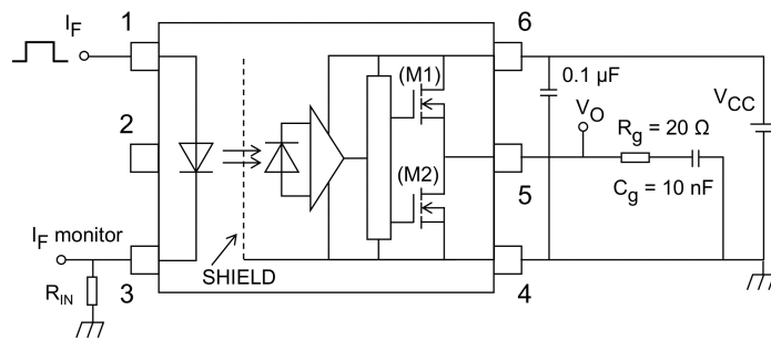
Fig. 13.1.7 Switching Time Test Circuit and Waveform
