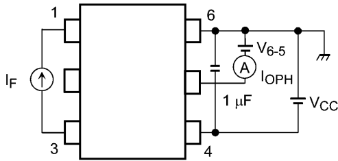
Fig. 13.1.1 I_{OPH} Test Circuit
