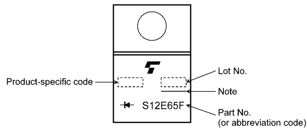
Fig. 7.1 Marking
