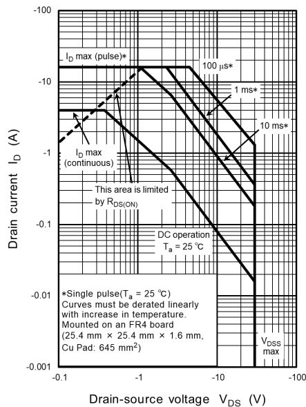
Fig. 9.10 Safe Operating Area
