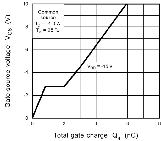
Fig. 9.8 Dynamic Input Characteristic
