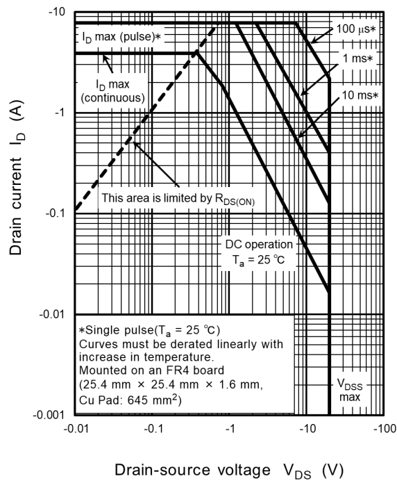
Fig. 8.9 Safe Operating Area
