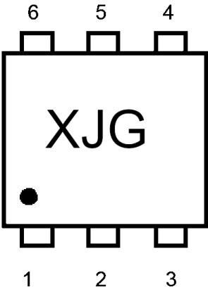
Fig. 7.1 Marking
