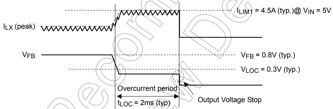
Figure 4 Overcurrent Operation
