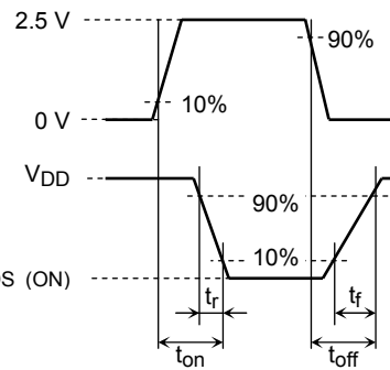
(c) V_{OUT}
