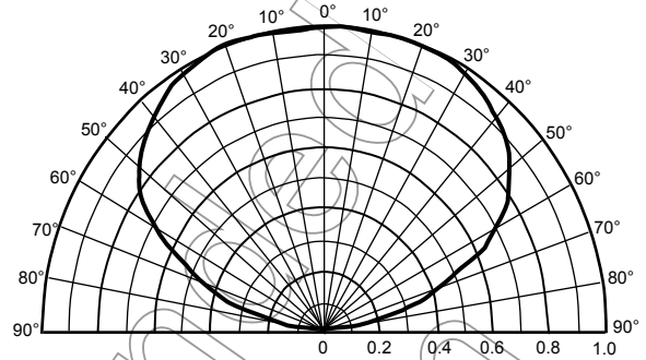
Horizontal to polarity Ta=25°C
