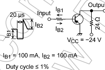
Fig. 5.2.1 Switching Time Test Circuit
