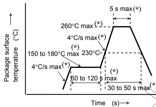
Temperature profile for Pb-free soldering (example)
