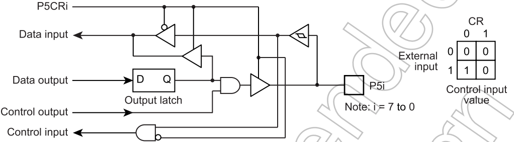
Figure 5-7 Port P5
