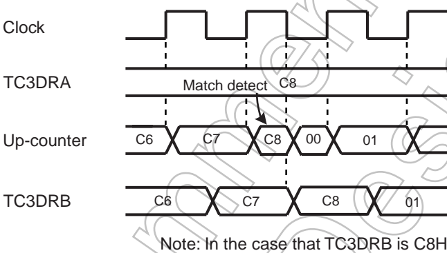
Figure 10-2 Auto-Capture Function
