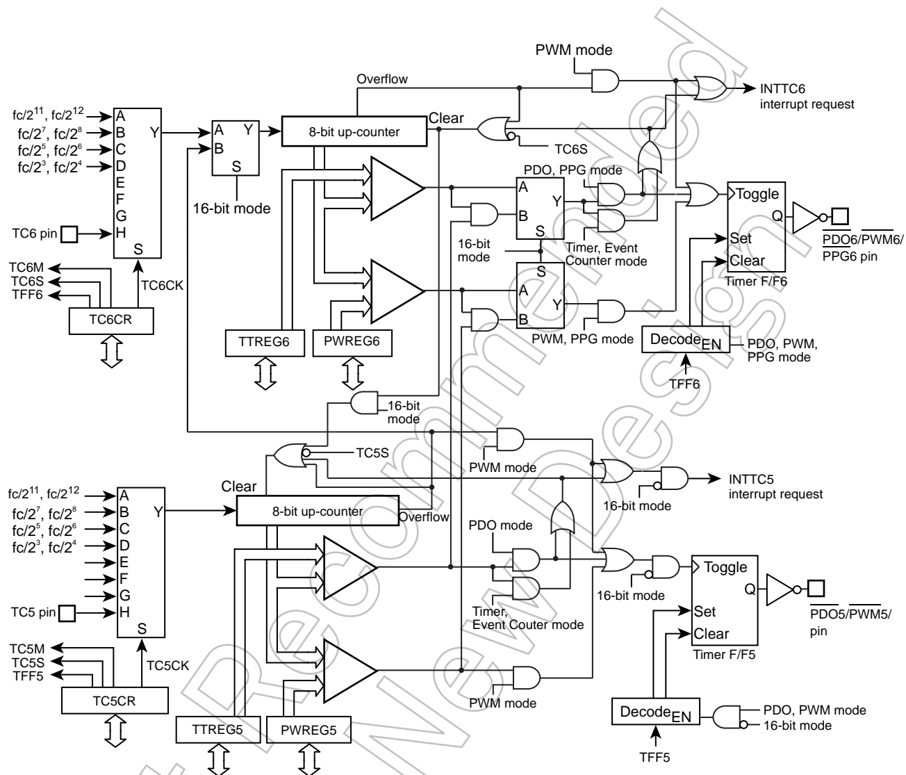
Figure 12-1 8-Bit TimerCounter 5, 6
