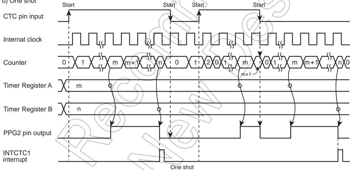
Figure 9-8 Two Register Both edges Trigger Start Mode Timing Chart
