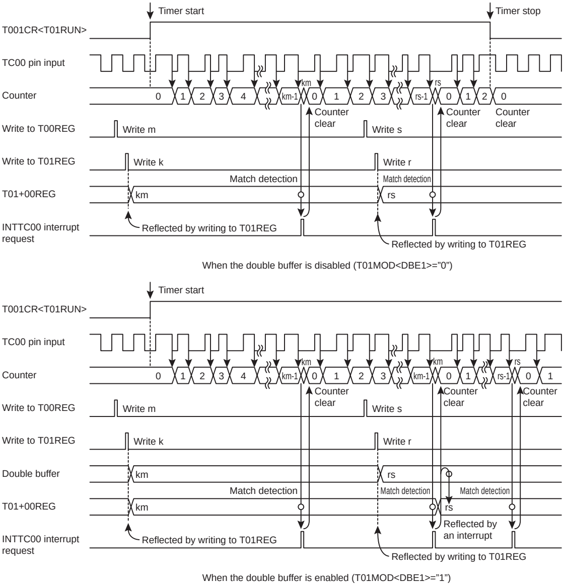
Figure 14-12 16-bit Event Counter Mode Timing Chart
