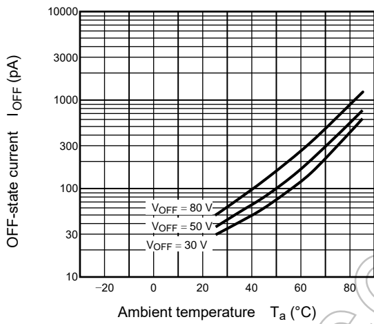
Fig.12.9 I OFF – T a
