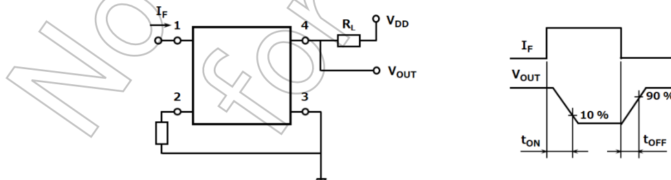
Figure 11.1 Switching Time Test Circuit and Waveform
