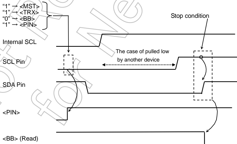
Figure 3.15.19 Stop condition generation (Multi master)
