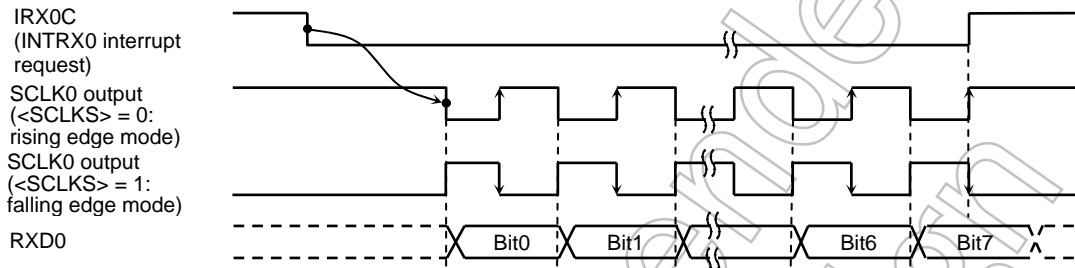
Figure 3.14.15 Receiving operation in I/O Interface Mode (SCLK0 Output Mode)
