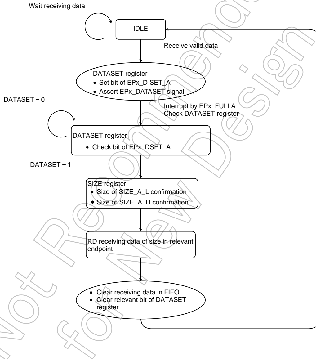
Figure 3.16.13 Receiving Sequence in Single Packet Mode
