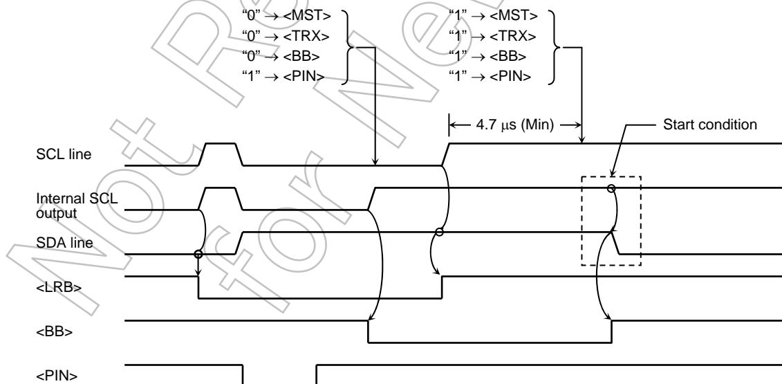
Figure 3.15.20 Timing chart for generate restart
