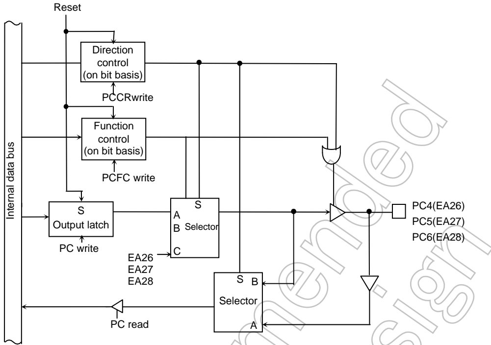
Figure 3.7.22 Port C4, C5, C6
