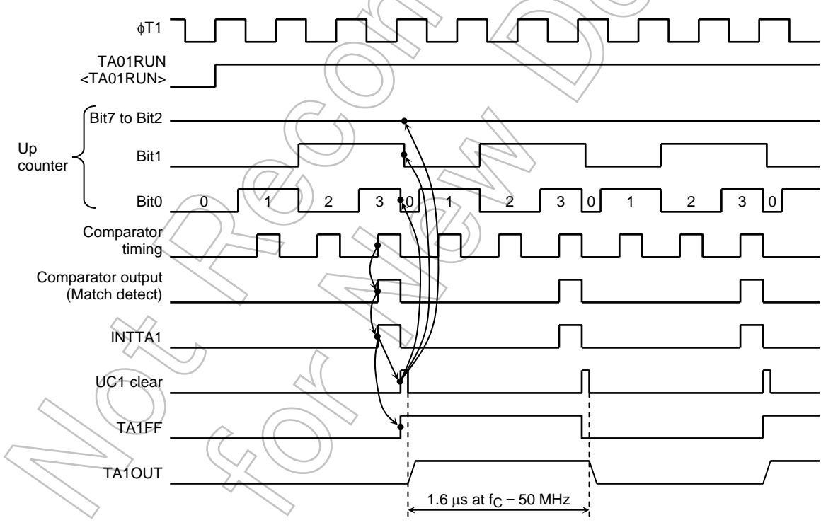
Figure 3.12.17 Square Wave Output Timing Chart (50% duty)
