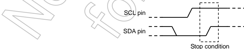
Figure 3.15.11 Stop condition generation
