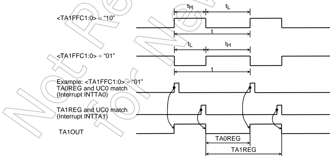
Figure 3.12.20 8-Bit PPG Output Waveforms
