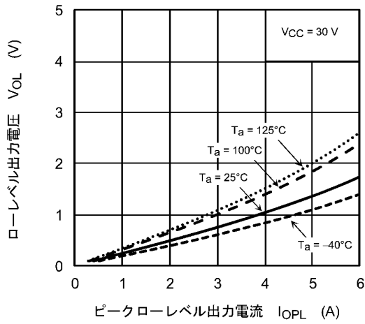
図 13.2.9 VOL - IOPL
