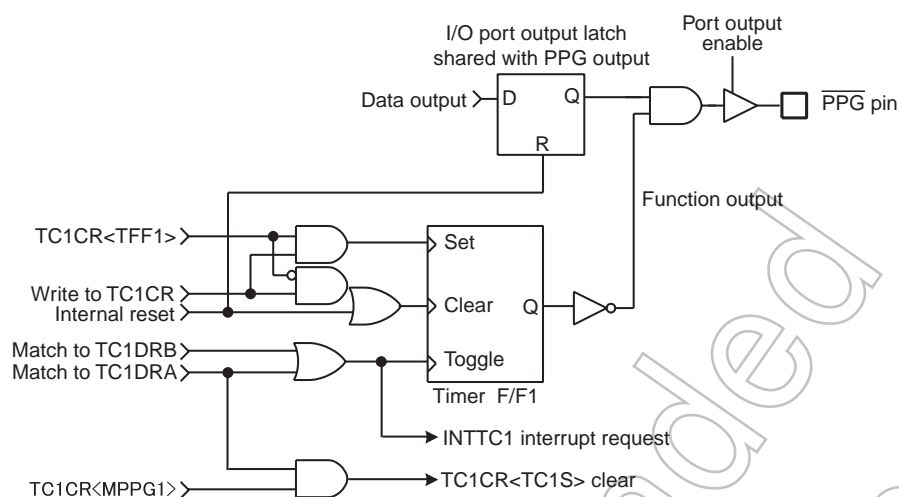
Figure 10-7 PPG Output
