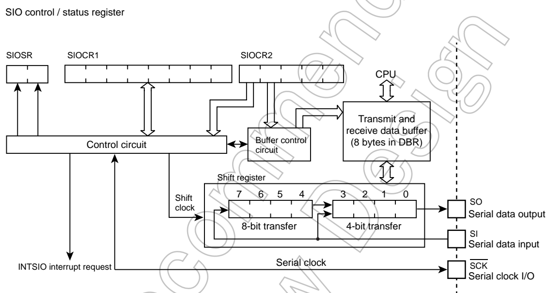
Figure 16-1 Serial Interface
