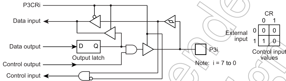
Figure 5-4 Port P3
