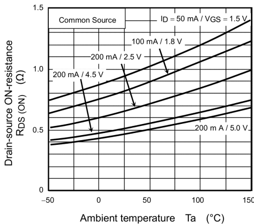
Fig. 7.5 R_{DS(ON)} - T_a
