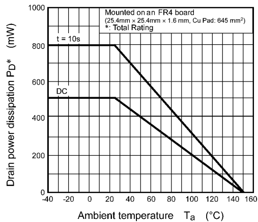
Fig. 7.12 P_D - T_a
