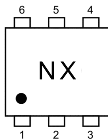
Fig. 6.1 Marking
