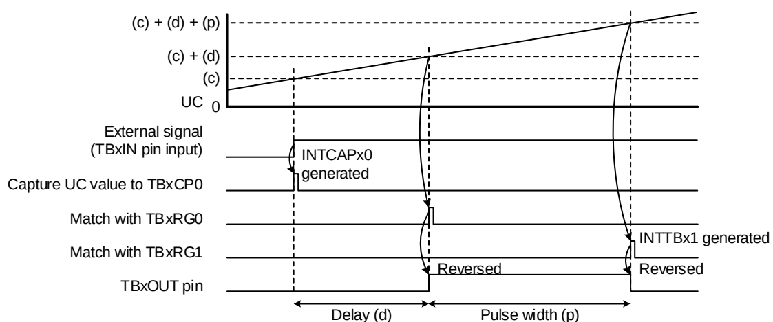
Figure 10.6 Square Wave Output from External Signal Using Free-running Counter (with Delay)
