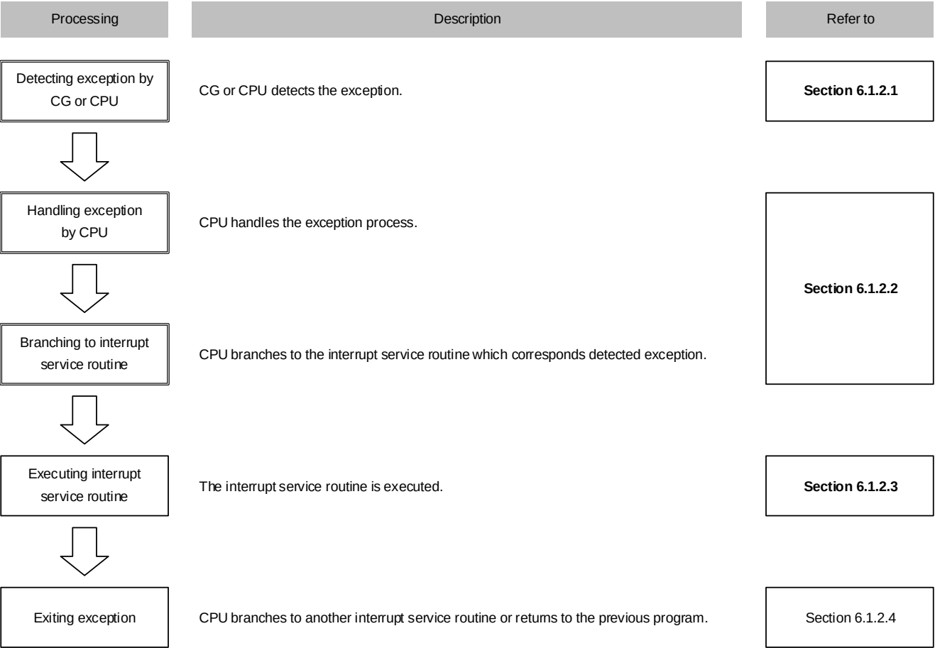
Figure 6.1 Handling Flowchart
