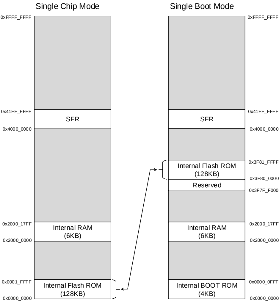
Figure 20.3 Memory Map
