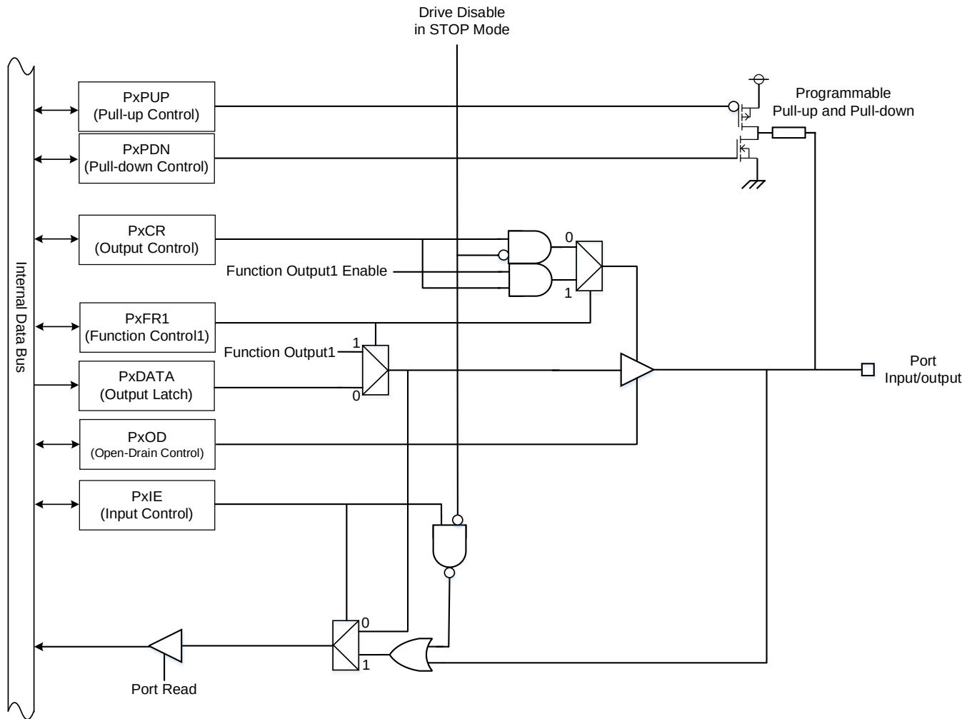
Figure 9.19 Port Type T19
