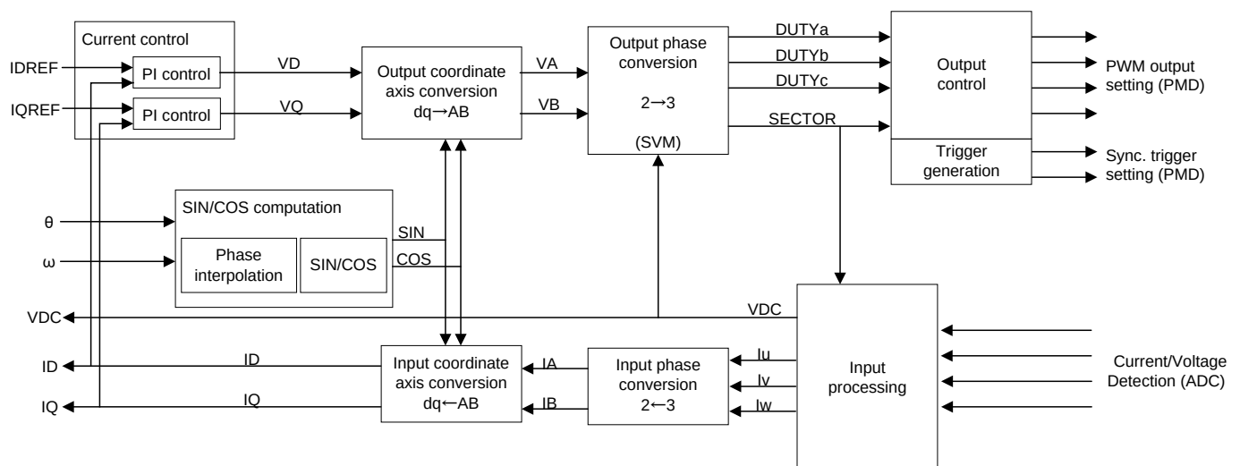
Figure 14.1 Block Diagram of Vector Control
