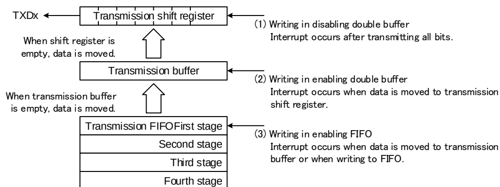
Figure 11.12 Transmission Operation Data Flow and Write Path
