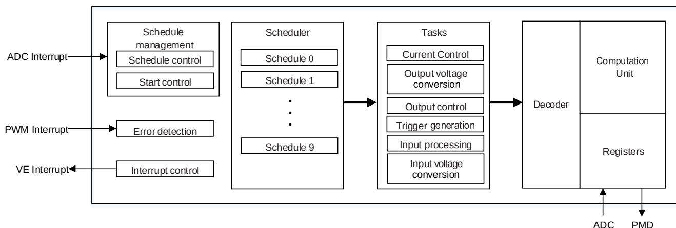
Figure 14.2 Configuration of VE
