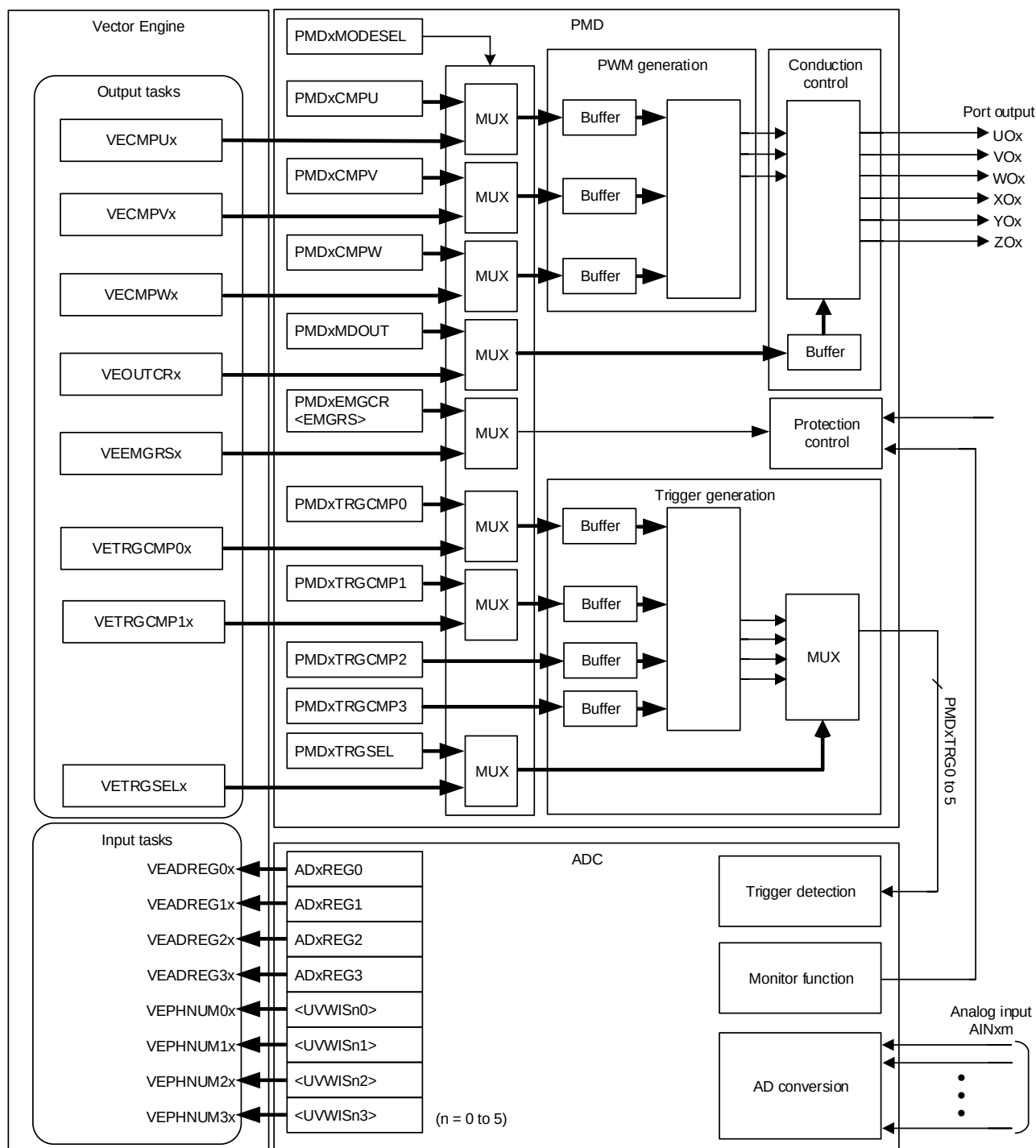
Figure 14.3 Interaction among VE, PMD and ADC
