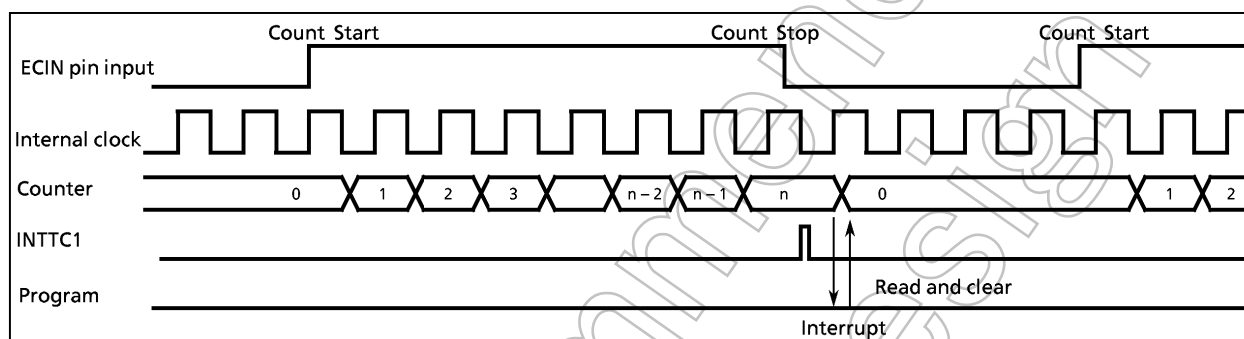
Figure 2-23. Pulse Width Measurement Mode Timing Chart (TC1CR2 &lt; SGEDG &gt; = "0")
