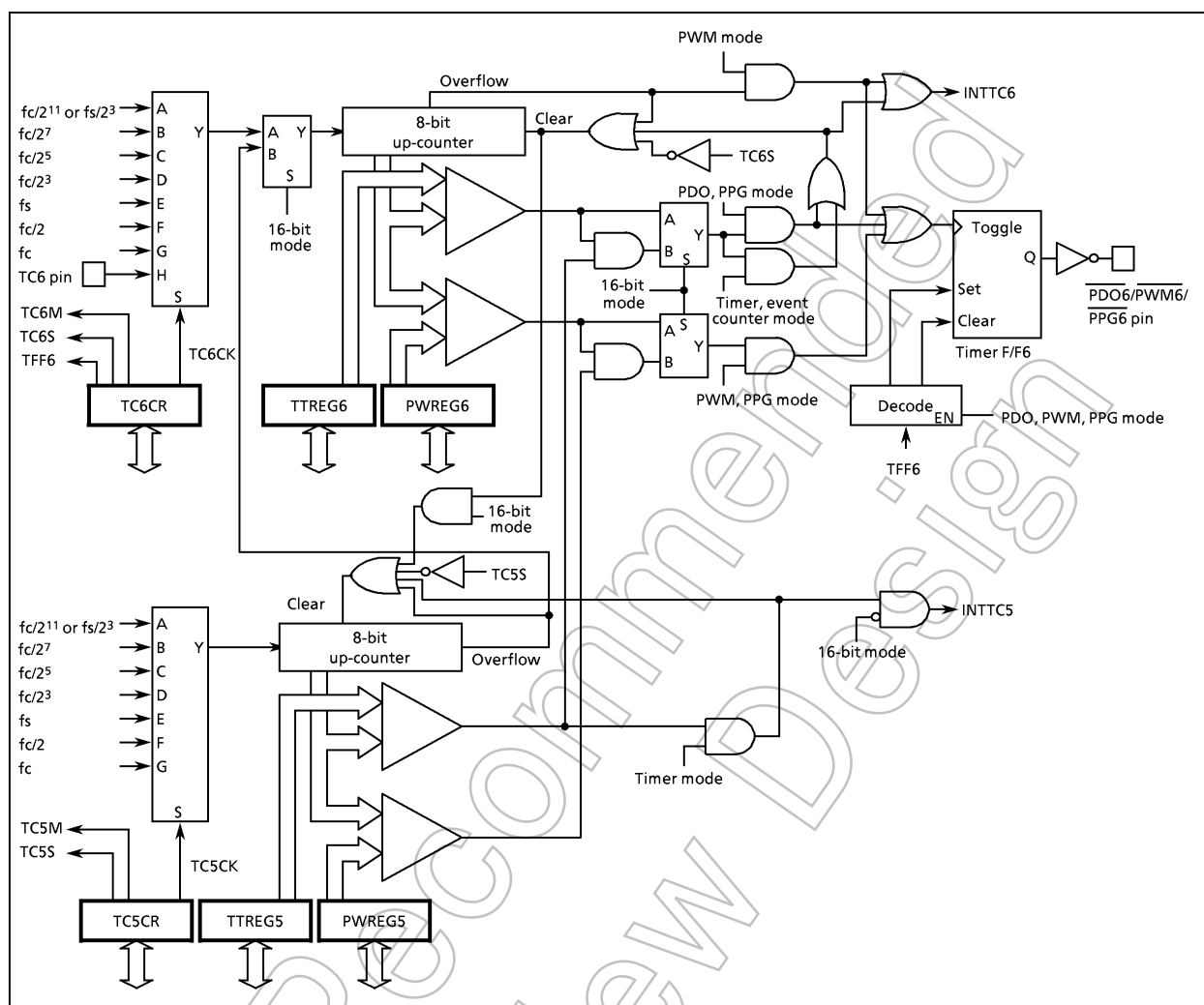
Figure 2-27. 8-Bit Timer 5, 6
