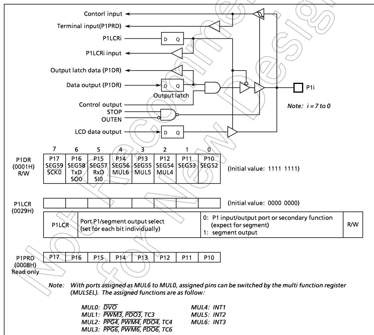
Figure 2-3. Port 1
