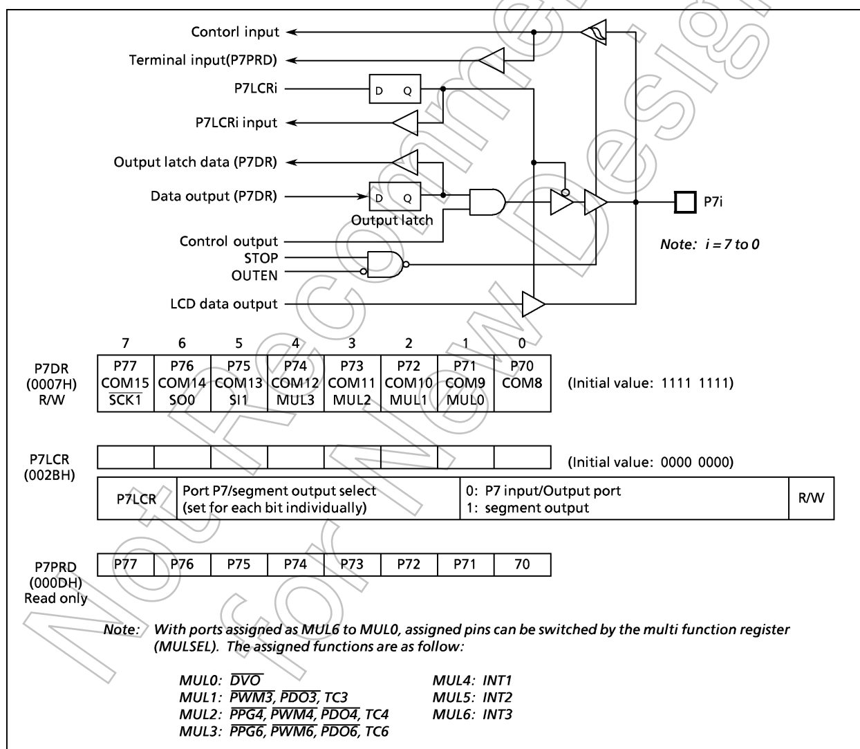
Figure 2-8. Port 7
