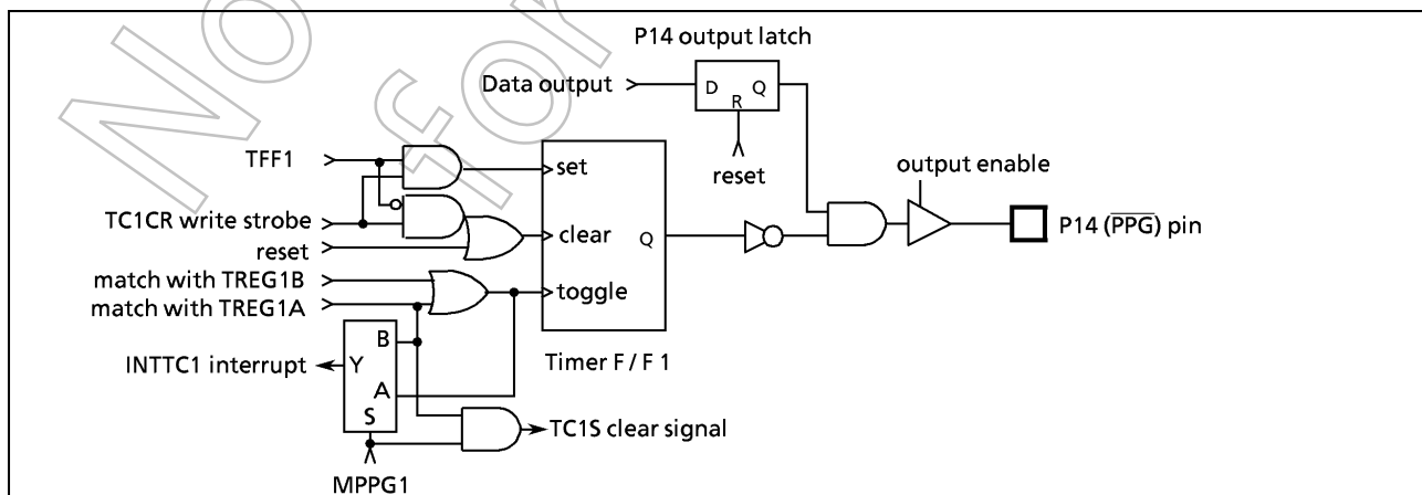
Figure 2-22. PPG Output
