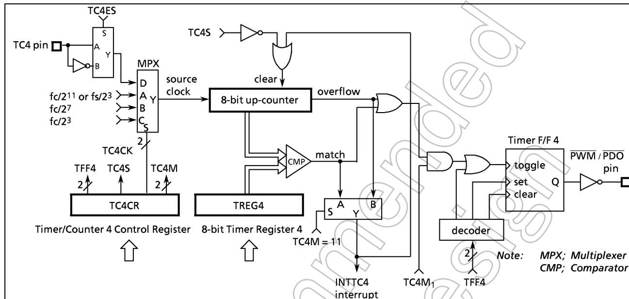
Figure 2-29. Timer/Counter 4
