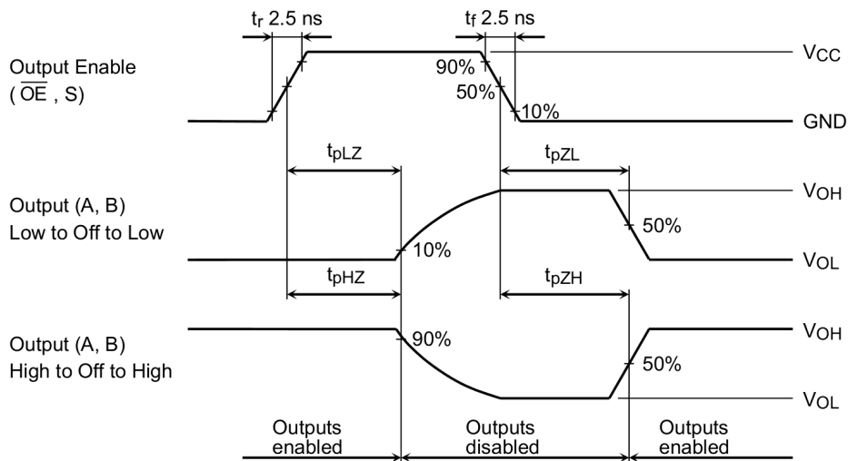
Fig. 11.8.1 AC Waveform t_{PLZ} , t_{PHZ} , t_{PZL} , t_{PZH}
