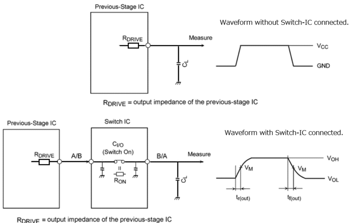
Fig. 12.1 Calculation Circuit
