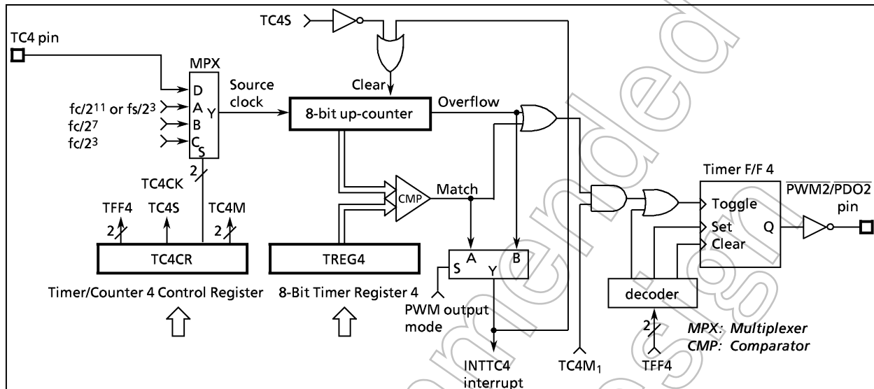
Figure 2-23. Timer/Counter 4
